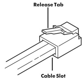
FIGURE 23: RJ-12 Modular Plug
